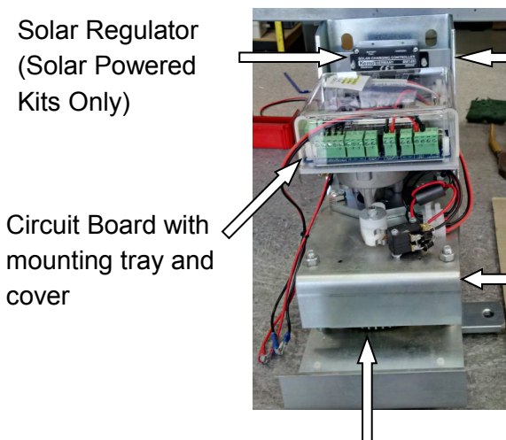
Motor Mounting Cradle
