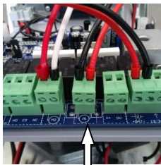
Motor M1 Terminals First Opening Gate / Last Closing Gate
